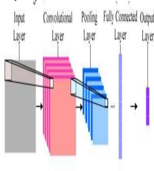
Fig 1 CNN Layers
