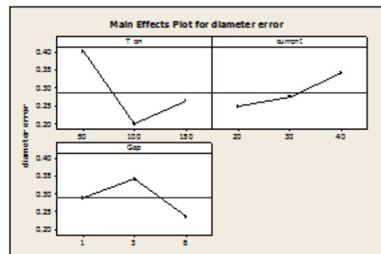
Fig.11 : The Effect of current, pulse on Time and on (Diameter error) using Brass electrode.
