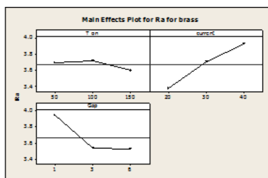
Fig.9 : The Effect of current, pulse on Time and on (Ra) using Brass electrode.
