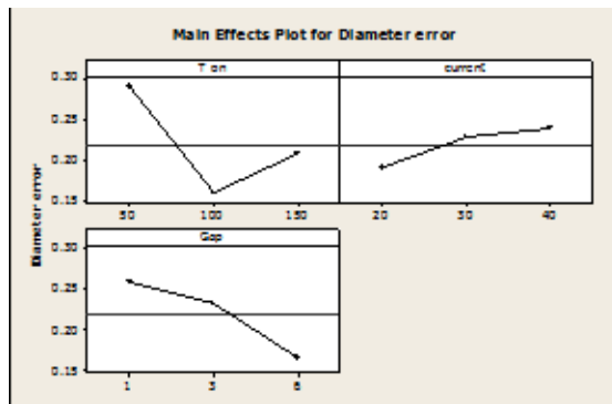
Fig.10 : The Effect of current, pulse on Time and Gap on (Diameter error) using copper electrode.
