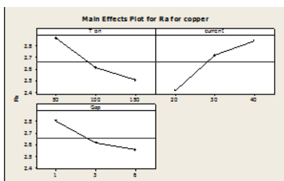
Fig.8 : The Effect of current, pulse on Time and Gap on ( Ra) using copper electrode.
