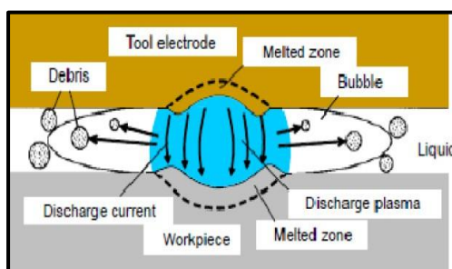
Fig.1 : Sparking occurs at closest points [3].
