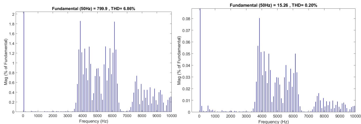
Fig 7. Output voltage and current THD of 17 level inverter with APD-PWM and modulation index is 1
