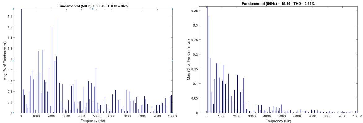
Fig 9. Output voltage and current THD of 17 level inverter with NLC-PWM and modulation index is 1
