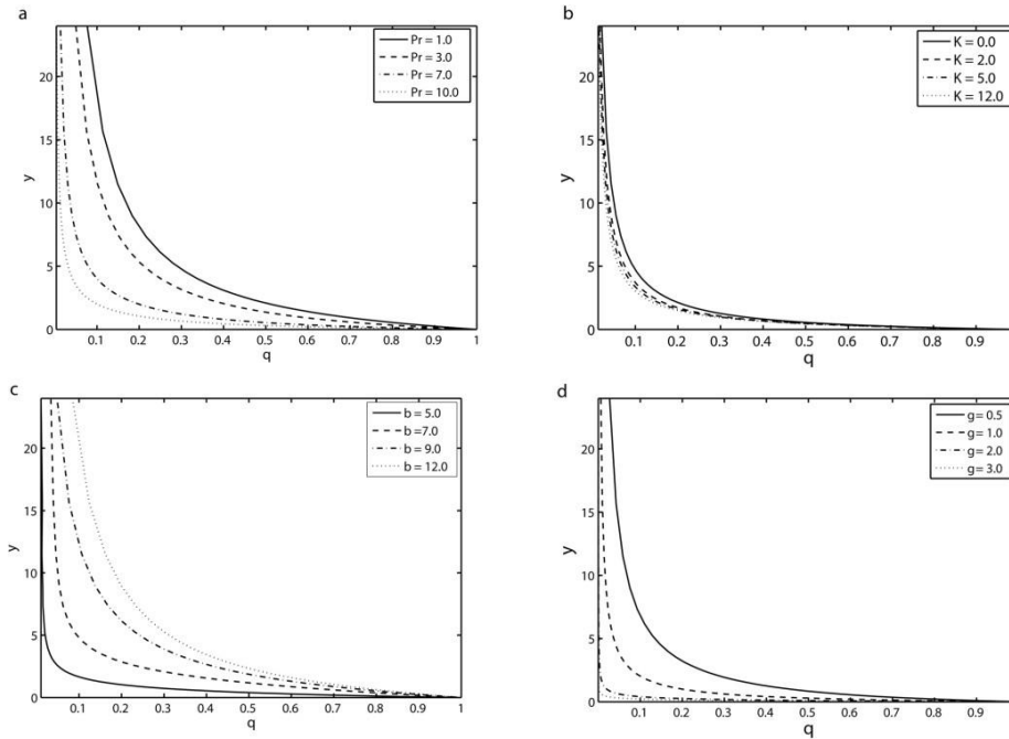
Fig 8. Transverse profiles of the temperature field \theta at the time point \tau = 8\pi : (a) effects of Pr with K = 0.2 , \gamma = 0.5 , S = 1 , \beta = 10 , (b) effects of K with \gamma = 1.5 , S = 0.1 , \beta = 12 and Pr = 1.5 and (c) effects of \beta with K = 0.2 , S = 1 , \gamma = 0.5 and Pr = 5 (d) effects of \gamma with K = 0.1 , S = 2 , \beta = 12 and Pr = 5 .
