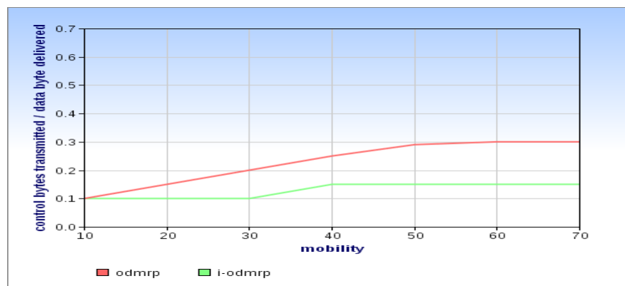
Fig. 6 mobility vs control bytes transmitted per data byte delivered.
