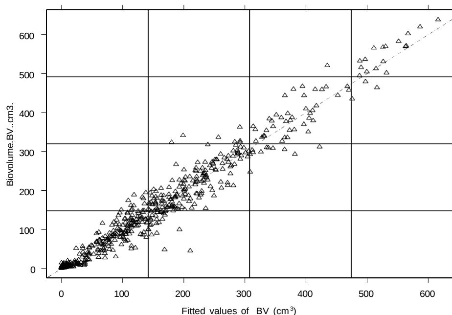
Figure 1. Correlation between observed and predicted maize stalk volume in Sauri, western Kenya
