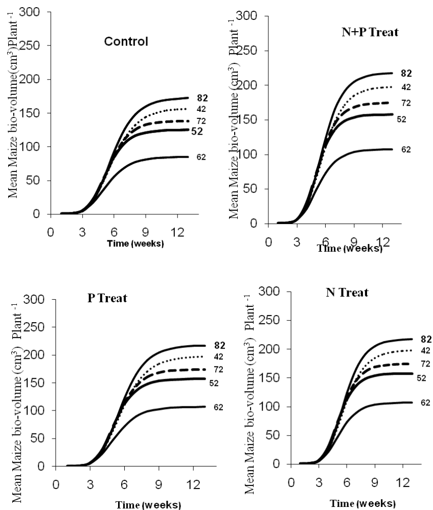
Figure 4: Effects of various fertilizer treatments in relation initial soil fertility status (Control) on maize in Sauri, western Kenya Key: Flat plots 82-Sauri-B, 42-Nyamninia – B, 72-Kosoro, 52-Silula, 62-Nyamboga
