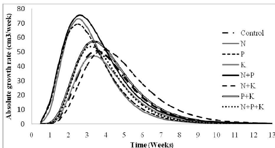
Figure 3. Observed variation of absolute growth rate of maize biovolume due to effects of applied fertilizer treatments in Sauri, western Kenya
