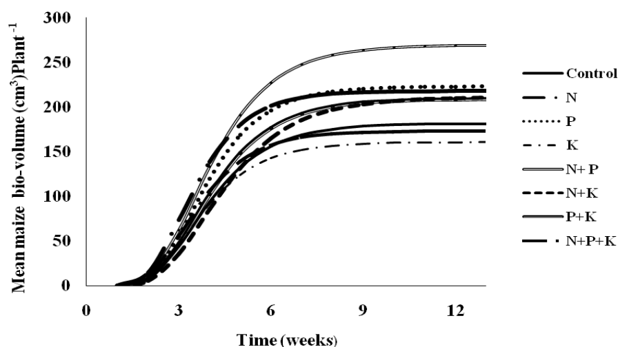
Figure 2 Effects of fertilizer application on maize stalk volume (biovolume) during the growing season in Sauri, western Kenya
