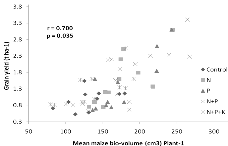
Figure 5. Correlation between maize grain yield and maximum stalk-volume growth in various villages in Sauri, western Kenya
