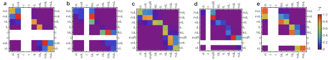
Figure 5: Degree of entanglement (4) between the 8 outgoing modes for the five typing frequencies of Fig.3. Here c indicates a complex mode; ul , nl , ll , nul are the non-optical modes.
