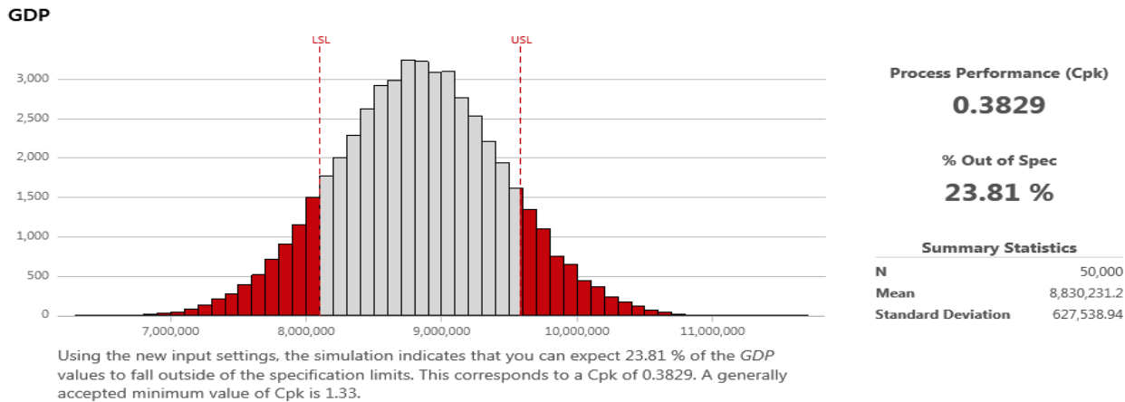
Figure 1.2: Parameter Optimization Results using Companion by Minitab
