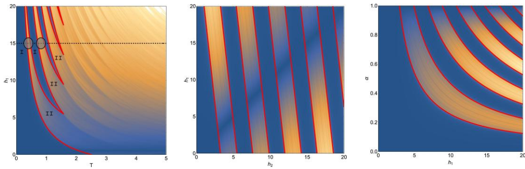
Figure 3: Density plots of the measure \square as a proxy of the non-locality of the Floquet Hamiltonian in the (T, h_1) -, (h_1, h_2) -, and (h_1, \alpha) -planes (from left to right). In all three figures, J = 1 , L = 10 , and N = 10001 . The other parameters are \gamma = 0.8 , h_2 = 0.5 , \alpha = 0.5 (left figure); \gamma = 0.2 , \alpha = 0.1 , T = 0.8 (middle figure); and \gamma = 0.2 , h_2 = 0.5 , T = 0.8 (right figure). The red lines separating the different regions are the predictions according to Eqs. (27). Note the local line h_1 = h_2 in the middle plot, which corresponds to a trivial quench-driven protocol for which the Floquet Hamiltonian is precisely the average one.
