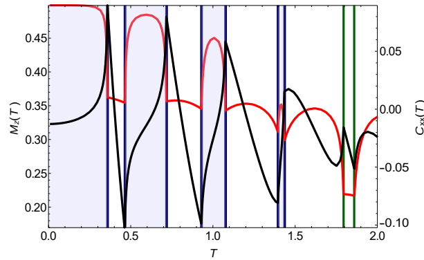
Figure 9: Synchronous value of the total magnetization M = \frac{1}{N} \sum_{i=1}^N S_i^z (red line) and correlator C_{xx} = \frac{1}{N} \sum_{i=1}^N S_i^x S_{i+1}^x (black line) along the dotted line h_1 = 15 in Fig. 1. The transitions from local to non-local regions are accompanied by the presence of non-analyticities. The vertical green lines correspond to non-analyticities inside non-local regions.
