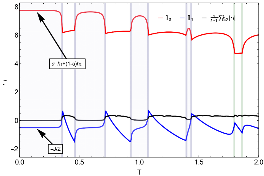
Figure 4: Effective couplings A_A as a function of the period. The red line shows the effective on-site magnetic field A_0 , the blue line the effective nearest neighbours interaction A_1 , and the black one the average strength of the remaining effective couplings. The latter becomes negligible inside the local regions indicated by the pale blue background.
