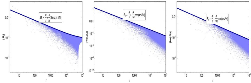
Figure 5: Effective couplings A_A (top panel) and B_A (real part in the central panel, imaginary part in the right one) as a function of distance in a non-local region, with J = 1 , \gamma = 0.8 , h_1 = 10 , h_2 = 0.5 , \alpha = 0.5 , T = 0.6 , and N = 1000001 . The dots indicate the absolute value of the corresponding coupling, while the continuous lines show the decaying envelope, which decays as A^{-1} up to finite size corrections.
