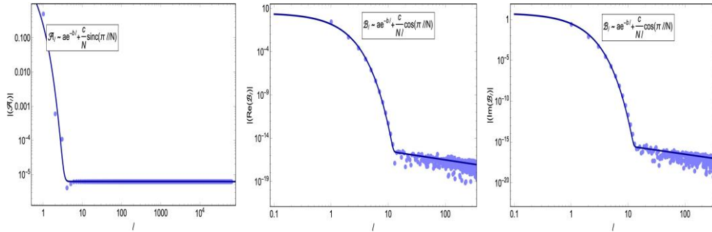
Figure 6: Effective couplings A_A (left panel) and B_A (real part in the central panel, imaginary part in the right one) as a function of distance in a local region, with J = 1 , \gamma = 0.8 , h_1 = 10 , h_2 = 0.5 , \alpha = 0.5 , T = 0.25 , and N = 1000001 . The dots indicate the absolute value of the corresponding coupling, while the continuous lines show in this case an exponential decay up to finite size corrections.
