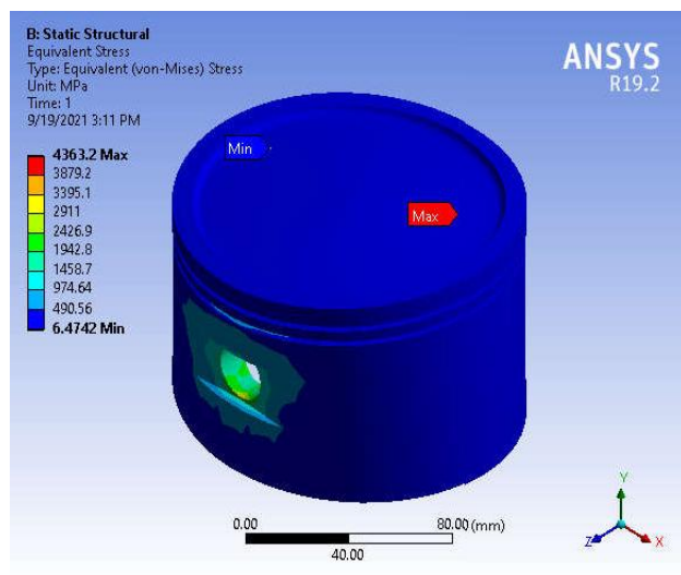
Figure 1.10 – Thermal stress distribution of titanium dioxide coated piston.
