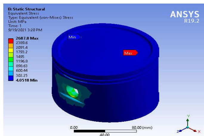
Figure 1.3 thermal stress distributions in piston (Validation)
