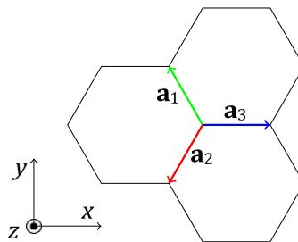
Figure 1: The honeycomb lattice with three different types of bonds and our choice of the global coordinate system.
