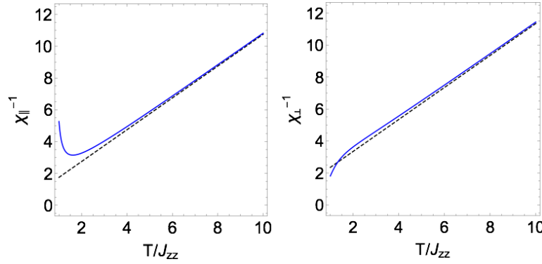
Figure 2: Susceptibilities versus temperature. The dashed black lines show the Curie-Weiss law, and the solid blue lines plot the inverse of equation (9). The parameters are chosen to be J_{zz} = 1, J_{\pm} = 0.9, J_{\pm\pm} = 0.2, J_{\pm z} = 0.1 . The susceptibilities in the plot, \chi_{||} and \chi_{\perp} , are in units of \mu_0 \mu_B^2 g_{||}^2 / 4k_B and \mu_0 \mu_B^2 g_{\perp}^2 / 4k_B , respectively.
