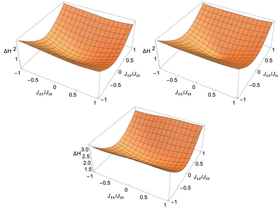
Figure 3: (Color online.) The dependence of \Delta H (defined in equation (14)) on J_{\pm\pm}/J_{zz} and J_{\pm z}/J_{zz} , with fixed values of J_{\pm\pm}/J_{zz} . Left: J_{\pm\pm}/J_{zz} = 1 , middle: J_{\pm\pm}/J_{zz} = 0.2 , right: J_{\pm\pm}/J_{zz} = -0.5 . In the first two panels, the linewidths are minimal at the “most isotropic” points J_{\pm\pm} = J_{\pm z} = 0 . In the right panel, we depict the case J_{\pm\pm}/J_{zz} < 0 , where the in-plane exchange is ferromagnetic. The linewidths \Delta in the three plots are in the units \mu_B g(\theta)/\sqrt{2} .
