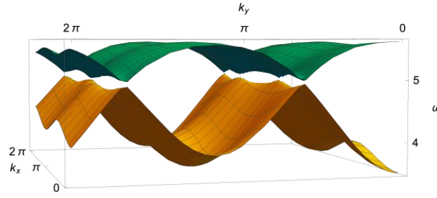
Figure 6: (Color online.) The two spin wave bands \omega_{\pm} when a strong in-plane field is present. The parameters are chosen J_{zz} = 1 ; J_{\pm} = 0.9 ; J_{\pm\pm} = 1 ; J_{\pm z} = 0.3 ; v = 5 .
