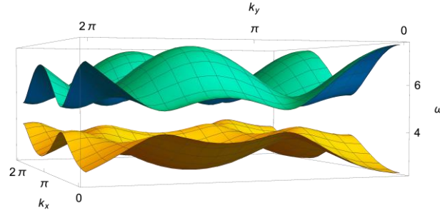
Figure 4: (Color online.) The two spin wave bands \omega_{\pm} when a strong field in the z -direction is applied. The parameters are chosen as J_{zz} = 1; J_{\pm} = 0.9; J_{\pm\pm} = 1; J_{\pm z} = 0.3; u = 5 .
