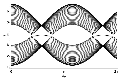
Figure 5: Edge state in a cylindrical geometry. The y -direction is periodic, while x -direction contains 50 sites. The parameters are J_{zz} = 1, J_{\pm} = 0.9, J_{\pm\pm} = 0.6, u = 4 .
