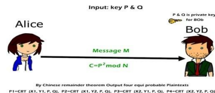
Fig. 2 Proposed Algorithm
