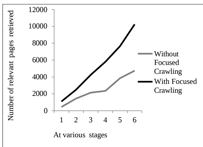
Fig. 7 The performance of the Crawler for the Anchor Text 'Java AWT'
