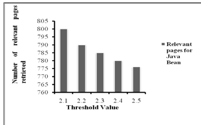
Fig. 4 Number of Relevant Pages Retrieved for the Topic 'Java Bean' on Different Threshold Values
