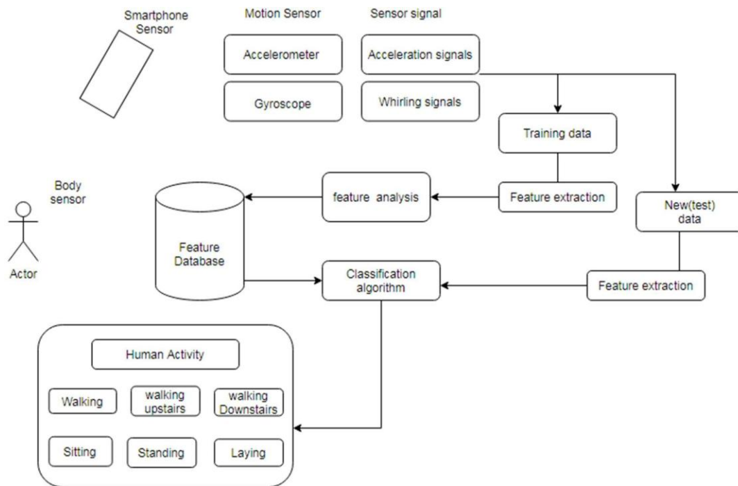
Fig 1.2 Flow diagram of Human Activity Recognition
