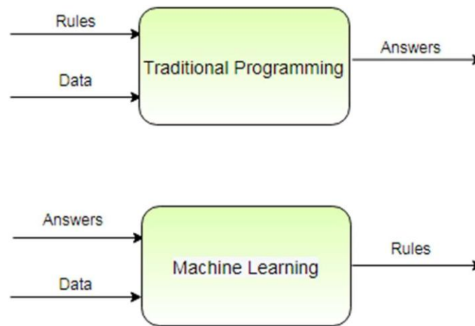
Fig 1.0 Difference in traditional programming and machine learning
