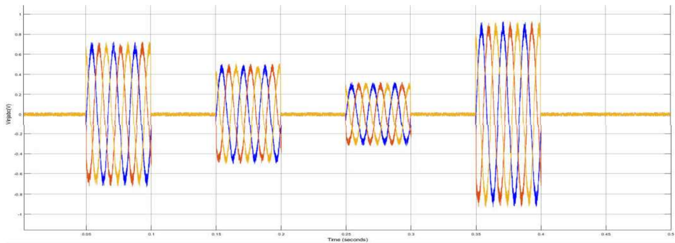
Figure:InjectedVoltage
