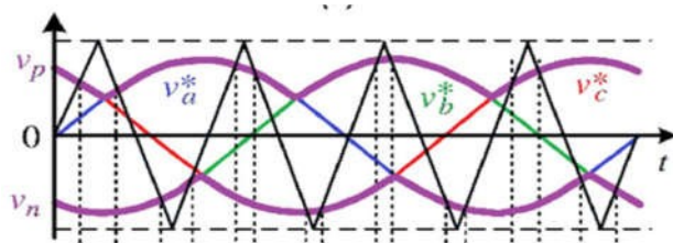
FigB:MBCMethod
