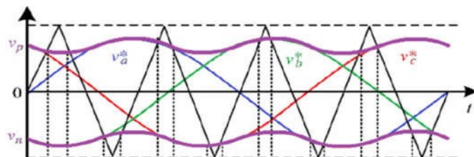
FigC:MCBCMethod
