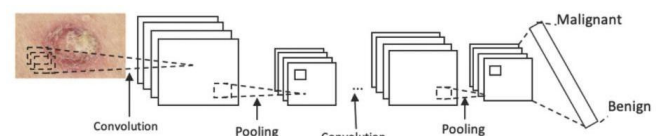
Fig. 6. The architecture of a typical convolutional neural network
