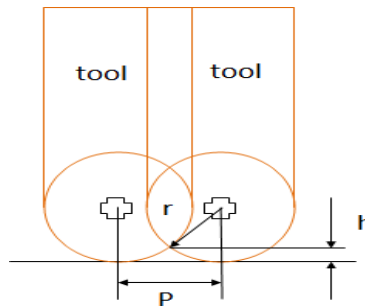
Figure (2): The workpiece machined showing the side steps
