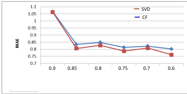
Figure 6 Ranking Error
