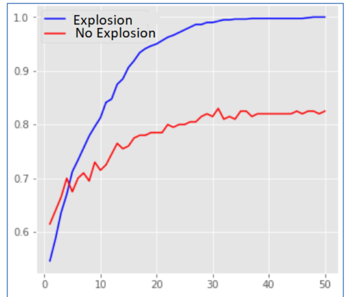
Figure 1 Accuracy comparison
