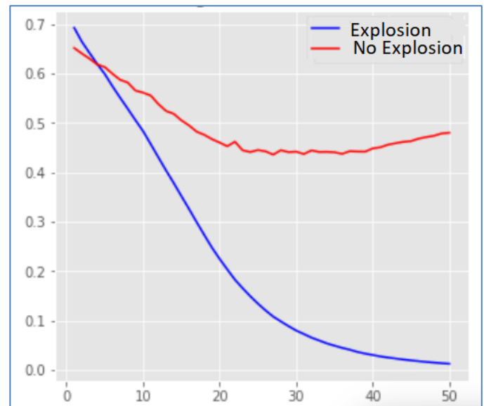
Figure 2 Loss Comparison
